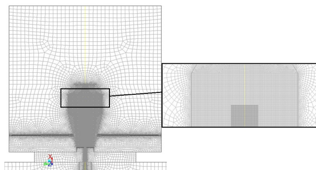
Figure 4.2: Grid used in Two Dimensional CFD simulations
