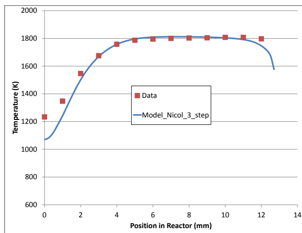
Figure 4.3: Profile of temperature from reactor centerline to wall, measured and predicted by CFD for CH 4 combustion for exit gas O 2 of 6.6% (mole %, dry)
