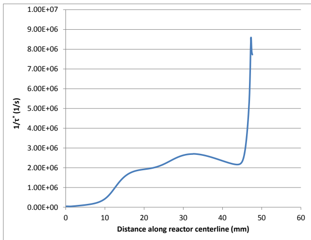
Figure 6.1: 1/\tau^* from reactor inlet to ceiling.
