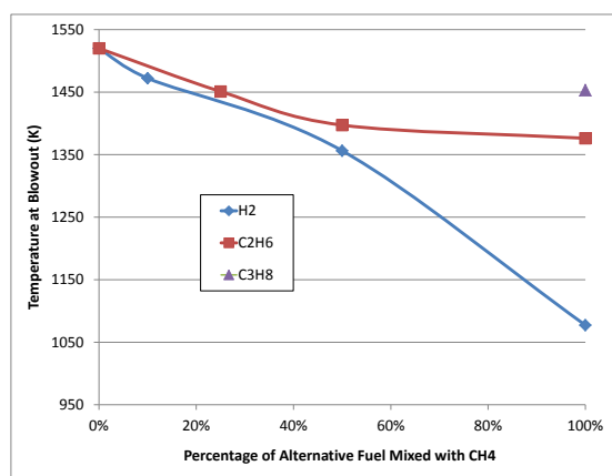
Figure 5.19: Experimentally determined blowout temperature for CH_4 mixed with increasing levels of H_2 and C_2H_6 . Blowout for pure C_3H_8 is shown for reference.
