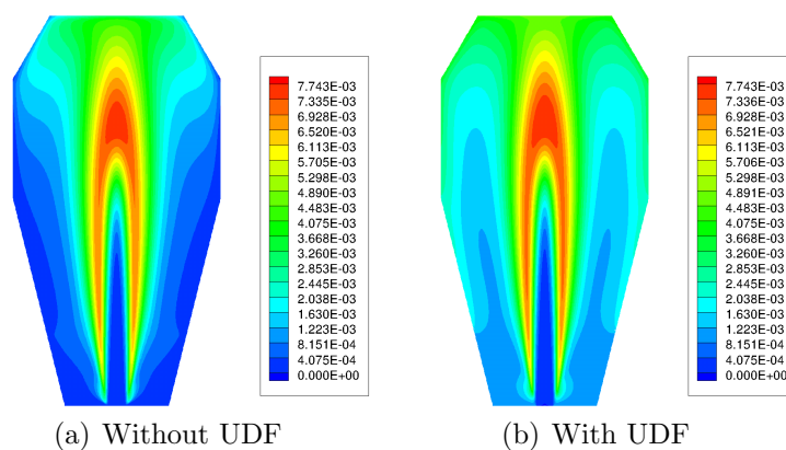
Figure 6.9: Contours of O predicted by CFD for \text{H}_2 combustion (mole fraction)
