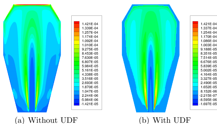
Figure 6.26: Contours of \text{NO}_x rate of production predicted by CFD for \text{H}_2/\text{CO} combustion ( \text{kmoles}/\text{m}^3\text{-s} ).
