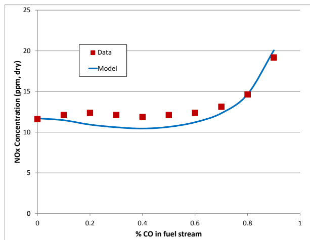
Figure 5.47: \text{NO}_x concentration as a function of CO concentration in the fuel stream for a fuel mixture of \text{CH}_4 and CO. Combustion temperature is kept constant at 1800 K.
