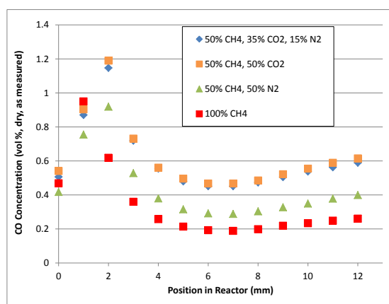
Figure 5.10: \text{CO} concentration profile across the JSR for the Landfill and Digester Gases with pure \text{CH}_4 shown for reference
