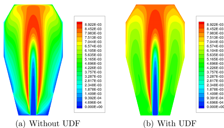
Figure 6.10: Contours of OH predicted by CFD for \text{H}_2 combustion (mole fraction)
