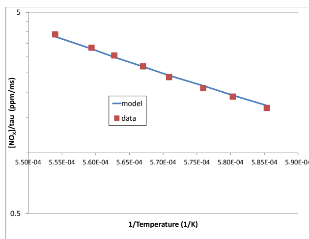
Figure 5.22: Net \text{NO}_X production rate for LPM \text{CH}_4 combustion showing both experimental and modeling results.
