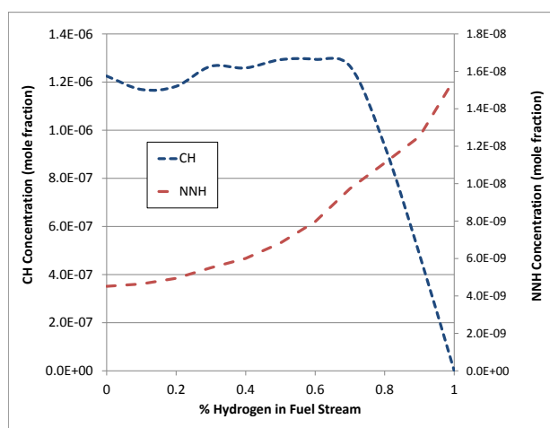
Figure 5.38: CH and NNH concentration in the turbulent flame brush for H_2 mixed with CH_4 . Combustion temperature is kept constant at 1800 K.
