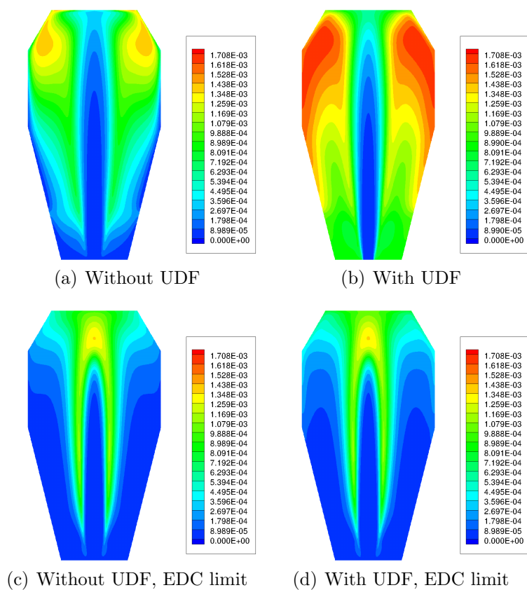
Figure 6.32: Contours of H atom for \text{CH}_4 combustion from the reduced GRI 3.0 mechanism both with and without the UDF at the default EDC conditions and at the EDC limit. (mole fraction)
